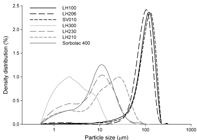
Fig. 3. PSD of lactoses measured dry dispersed at 2 bar disperser pressure. Black lines represent the coarse carriers (LH100, LH206 and SV010), light grey micronised lactose (LH300) and dark grey milled lactose grades (LH230, LH210 and Sorbolac 400). The data represents an average of five repeated measurements
