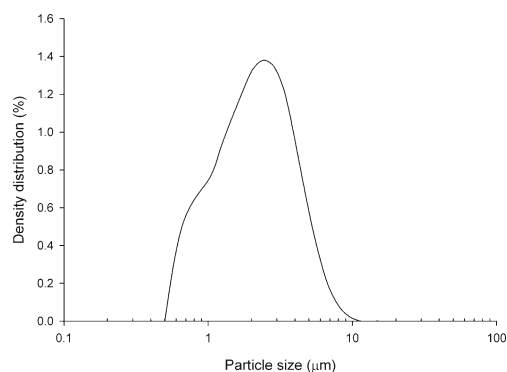
Fig. 1. PSD of budesonide measured by wet dispersion. The data represented is an average from five repeated measurements
