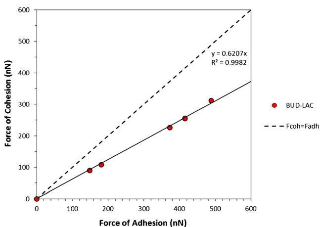
Fig. 2. Cohesive-adhesive balance (CAB) plot for the batch of budesonide. The dotted line represents F_{\text{coh}} = F_{\text{adh}} and corresponds to CAB value of 1
